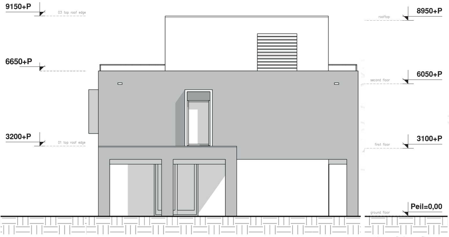
Right facade Scale 1 : 100
