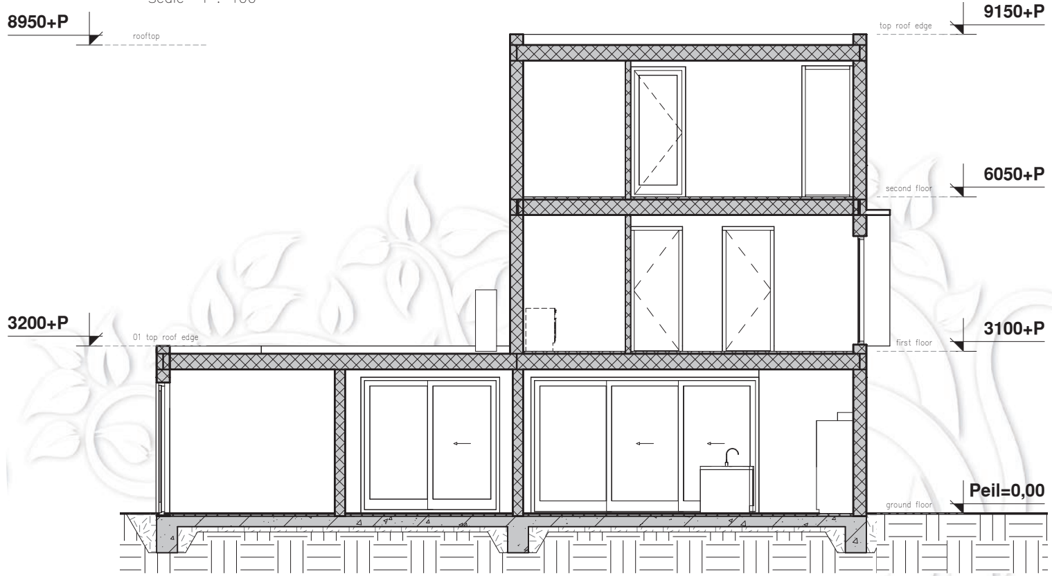
Section B
