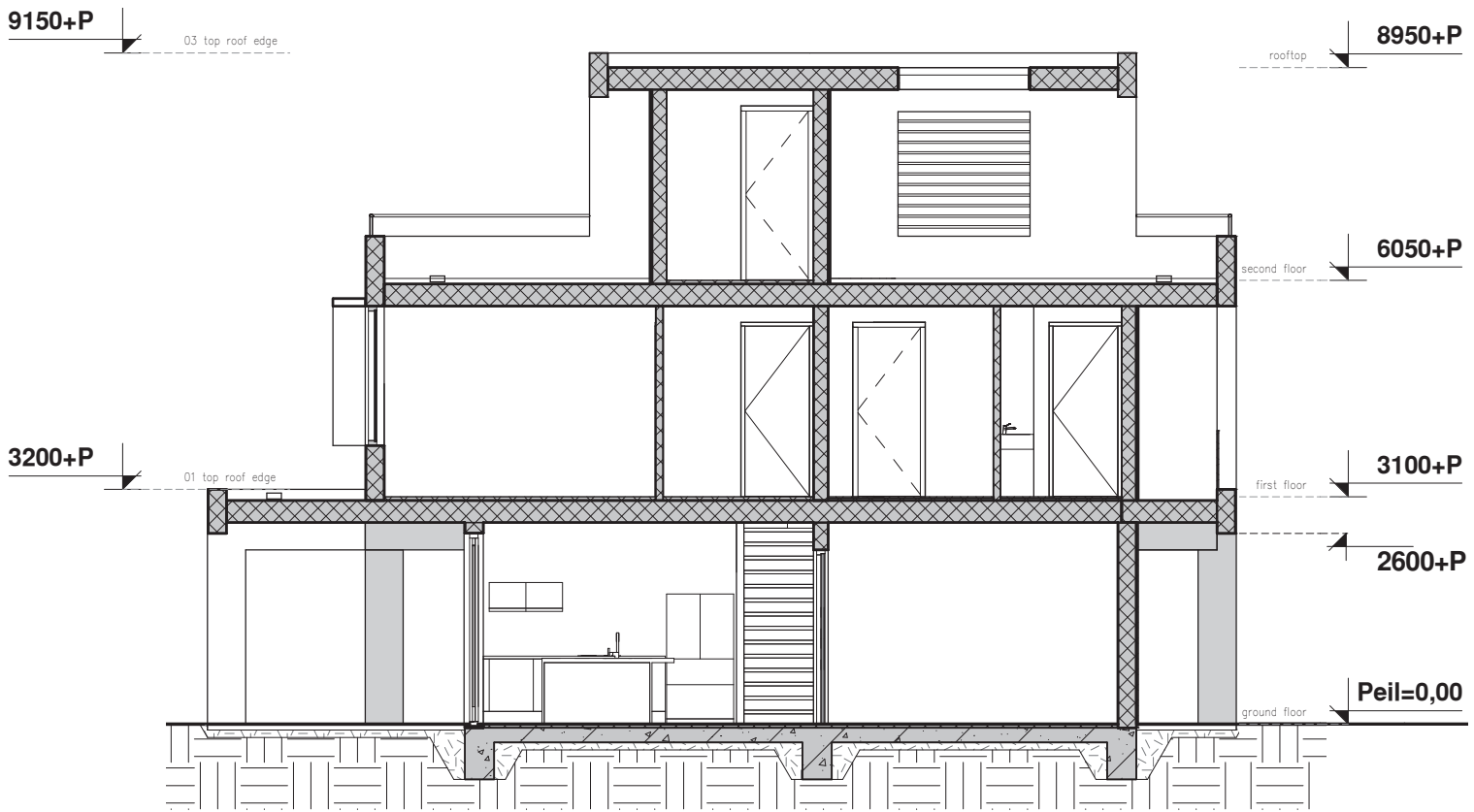
Section A
