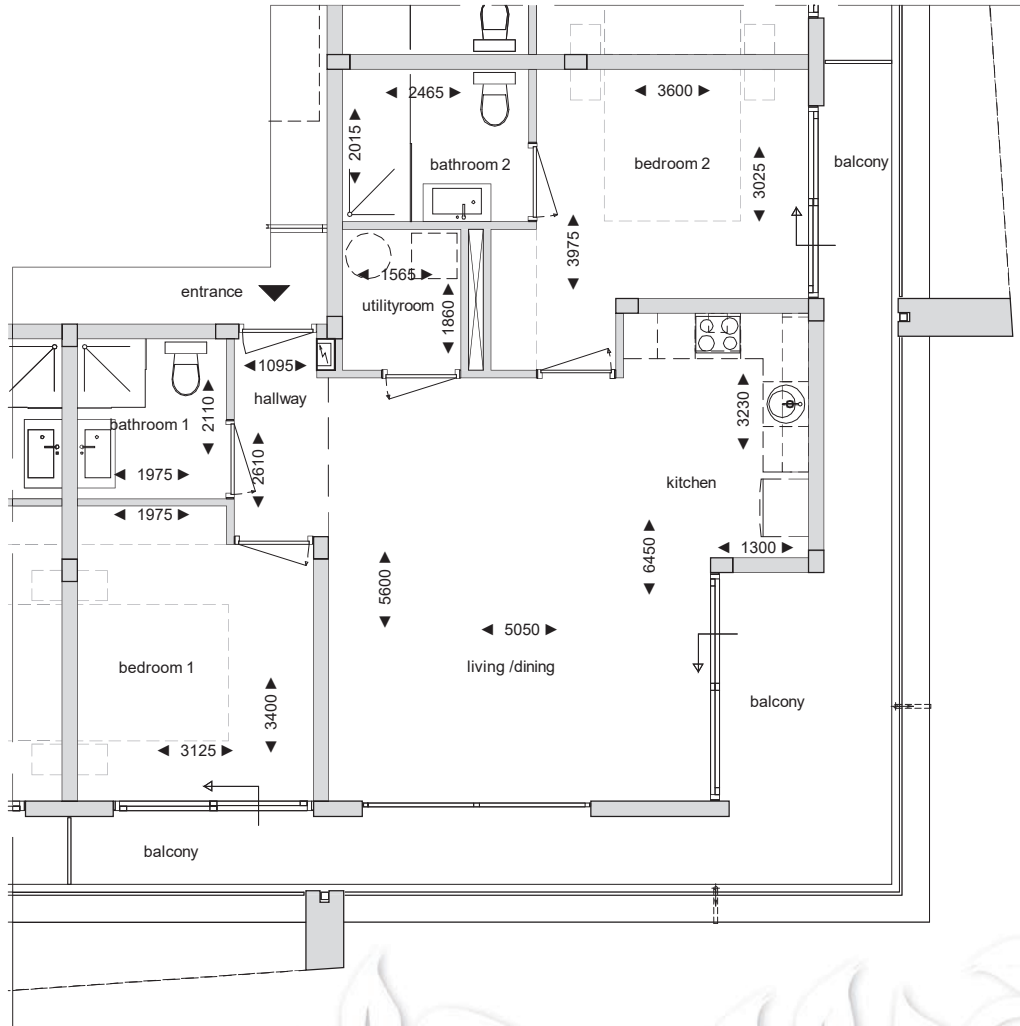
Second floor Condo 9 Scale 1:100
