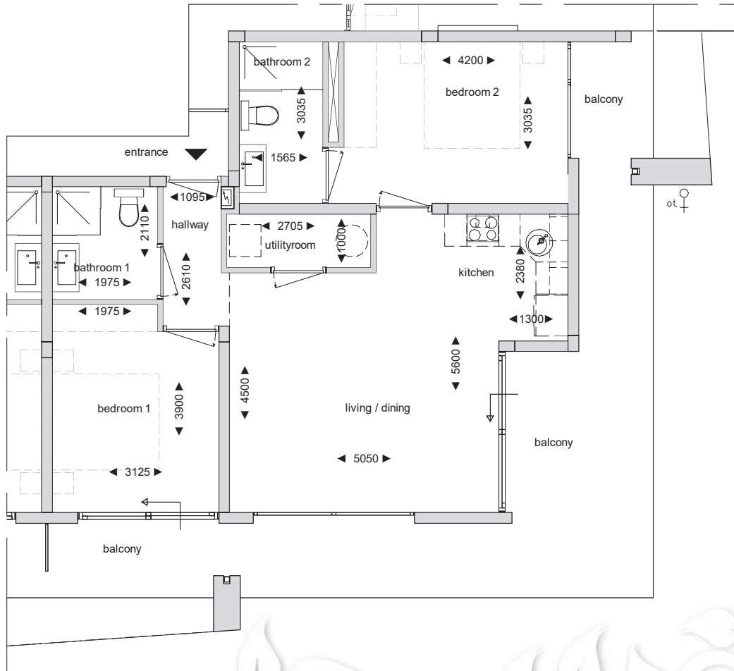
Ground floor Condo 1 Scale 1:100
